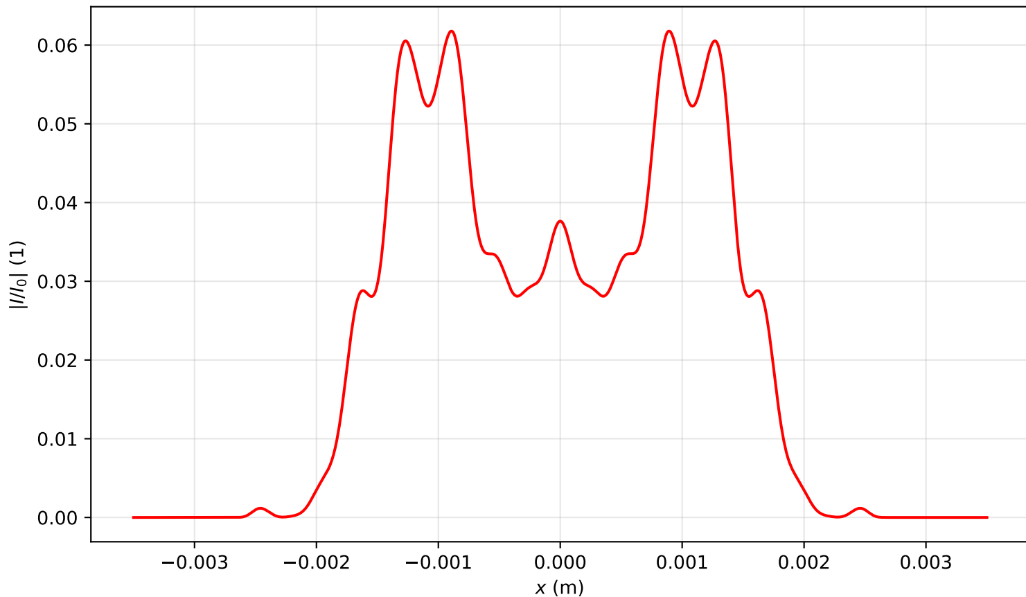
Intensity profile I(x, y = 0, z = 3.344)/I_0 , P_{in}=6.0P_{cr} , artificial time
